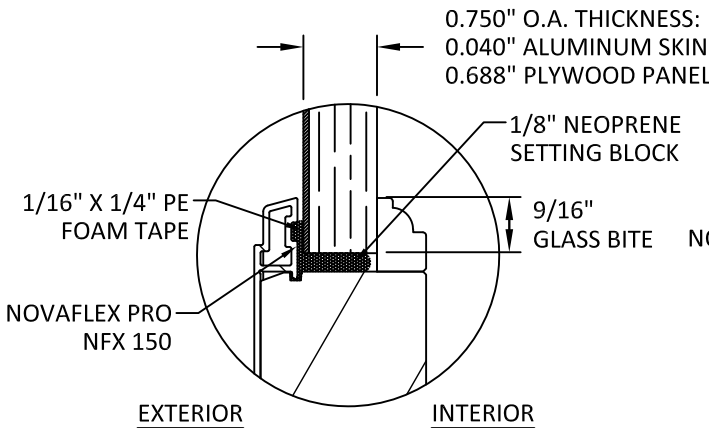
GLAZING DETAIL 2 PLYWOOD INFILL PANEL (G2)
