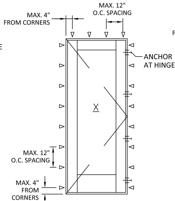
ANCHOR LAYOUT
