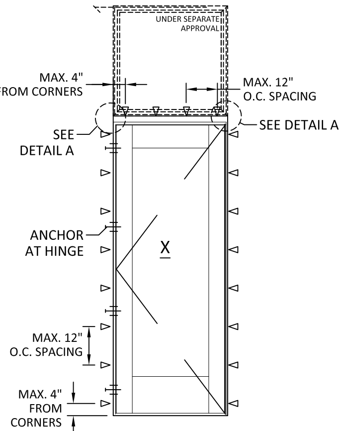
ANCHOR LAYOUT
