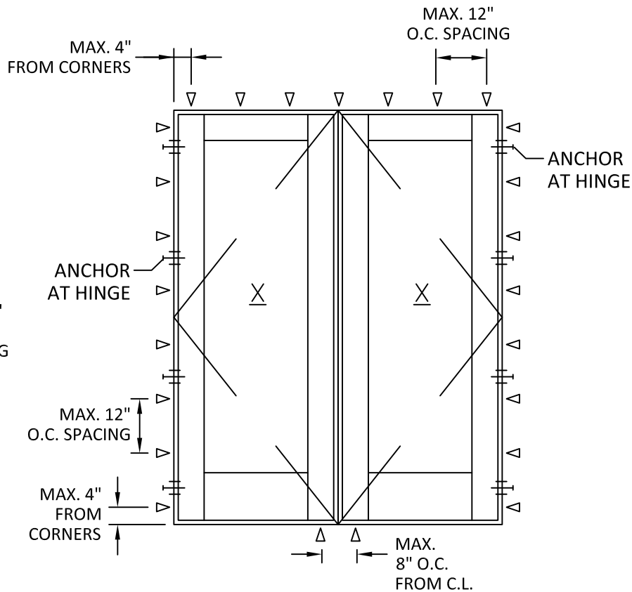
ANCHOR LAYOUT
