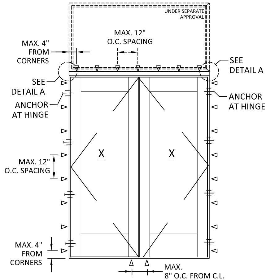
ANCHOR LAYOUT
