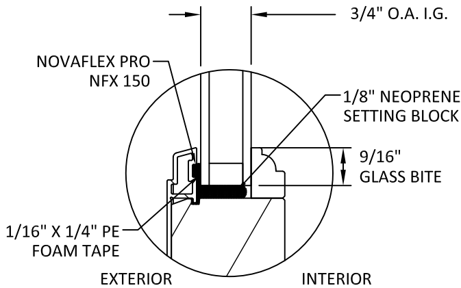
GLAZING DETAIL 1 3/4" IG GLAZING (G1)
