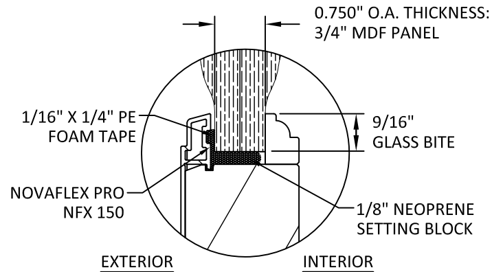
GLAZING DETAIL 4 MDF RAISED INFILL PANEL (G3)
