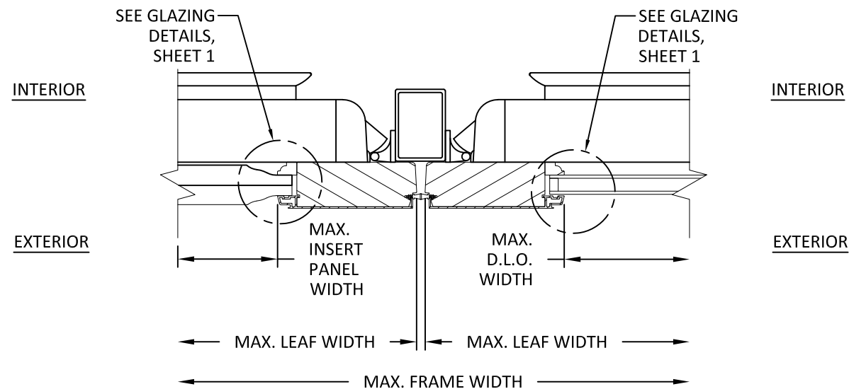
B HORIZONTAL SECTION 6 TYP. ASTRAGAL W/ EXIT DEVICE MULLION
